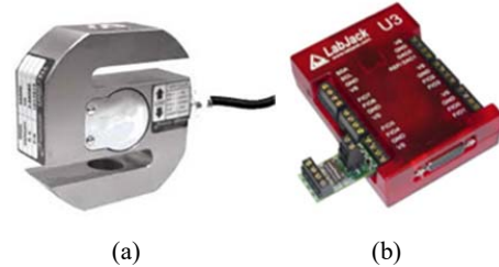
Fig. 7 (a) SS300 load cell and (b) Labjack U3 with amplifier
