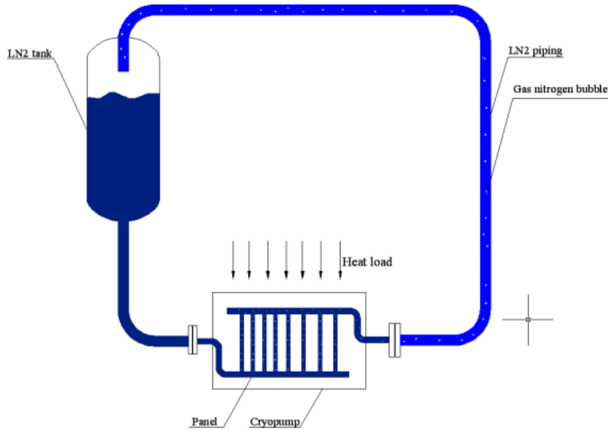
Fig. 1 Schematic drawing of gravity circulation loop system
