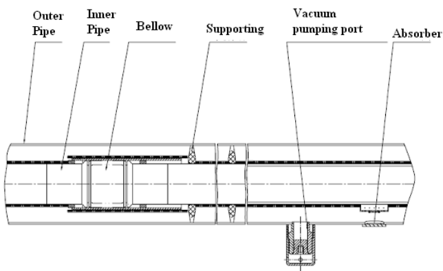
Fig. 3 Structure of vacuum insulation pipe
