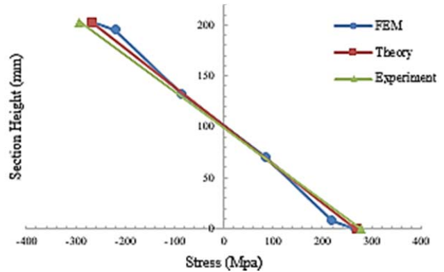
Fig. 5 Steel stresses in preflexion stage
