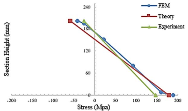
Fig. 6 Steel stresses after release stage
