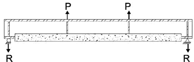
Fig. 3 Loading diagram at release stage
