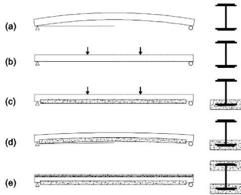
Fig. 1 Preflex beam construction stages
