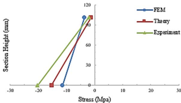
Fig. 7 Concrete prestress introduced by preflexion
