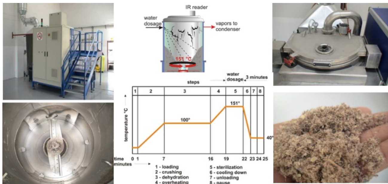
Fig. 2 OMPECO HCRW convertor system [10]
