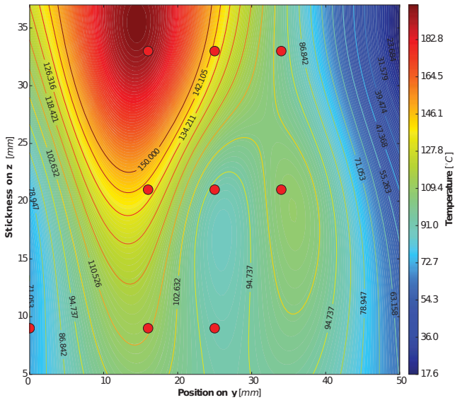
Fig. 13 Experimental 2D interpolated results between the transversal thermocouples on Z,Y at 100s of simulation for a current of 500A, a velocity of 140\text{ km} \cdot \text{h}^{-1} a,f a force of 60N
