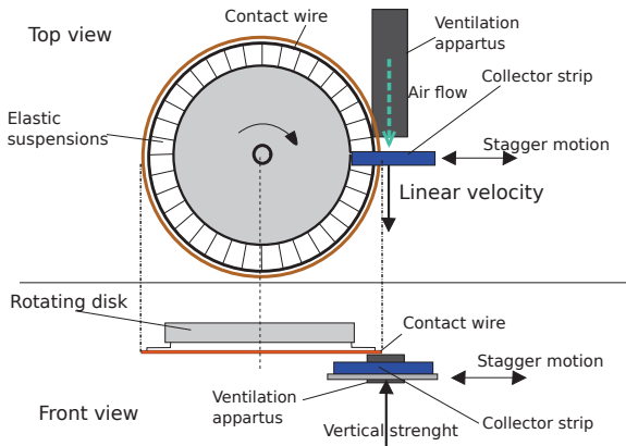
Fig. 9 Representation of the experimental bench
