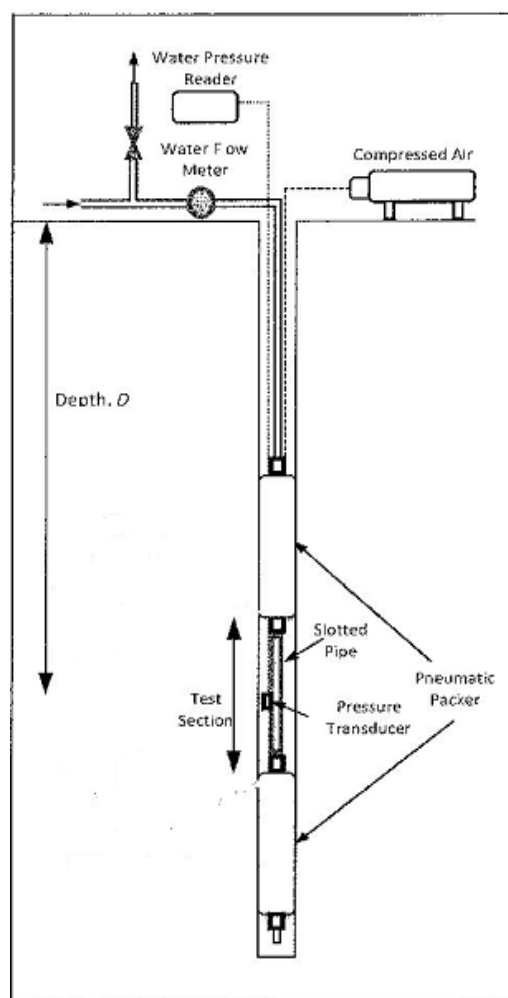
Fig. 1 Schematic diagram of Lugeon test
