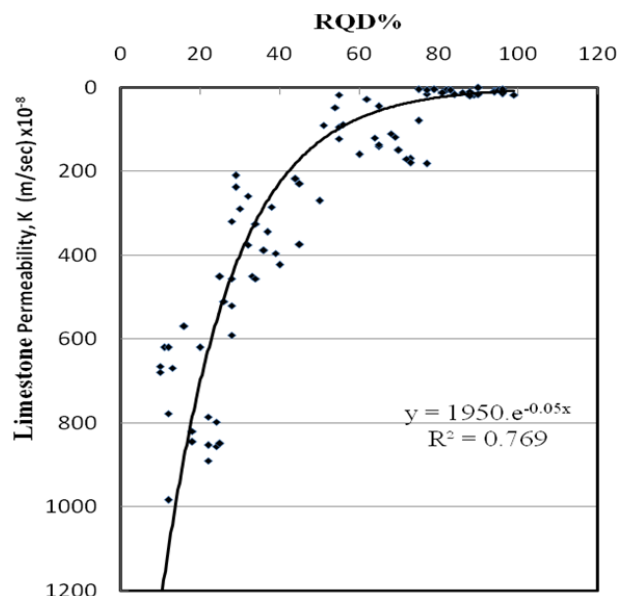
Fig. 5 Correlation between Limestone permeability and RQD index
