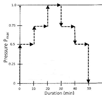
Fig. 2 Water pressure stages during Lugeon's test
