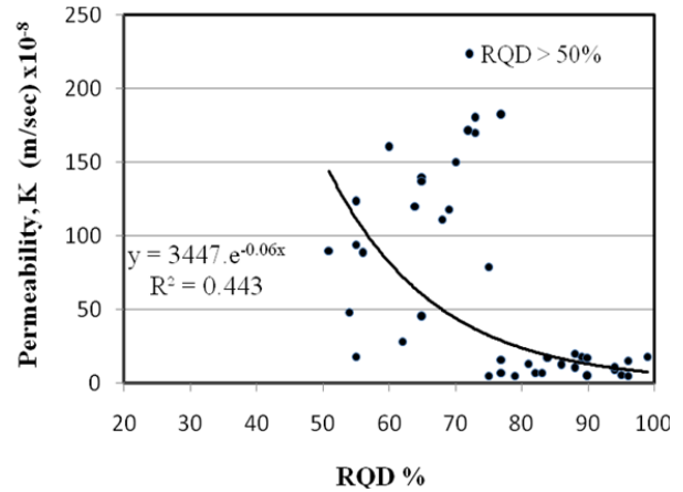
Fig. 4 (b) Correlation between limestone permeability and RQD index >50%
