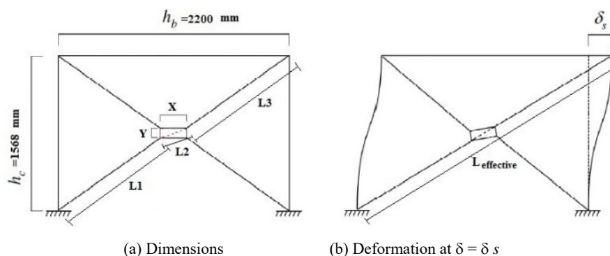
Fig. 5 Delayed wire-rope bracing using middle plate
