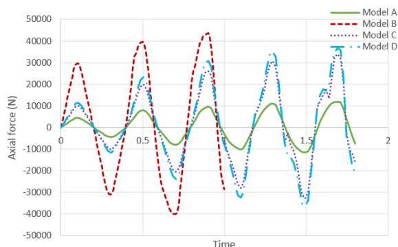
Fig. 10 Axial force to the left columns
