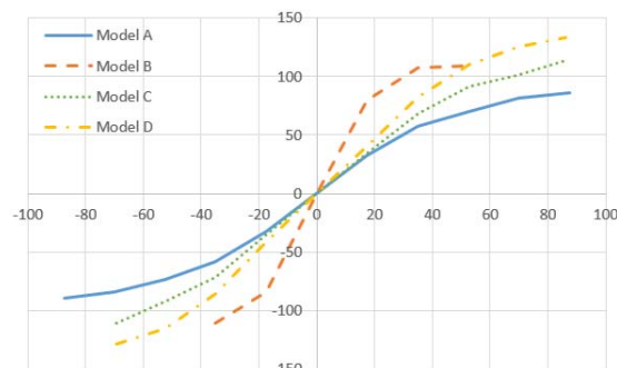
Fig. 8 Skeleton curves for frames A, B, C, and D
