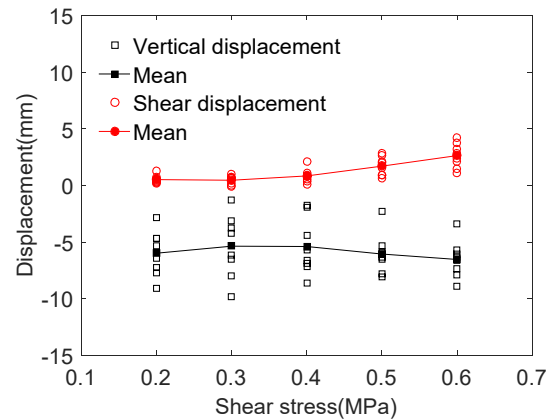
(b) Angular specimens
