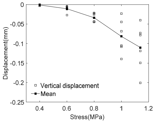
(a) Rounded specimens
