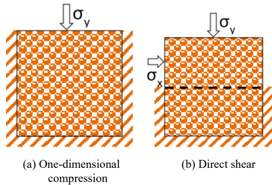
Fig. 2 Different boundary conditions
