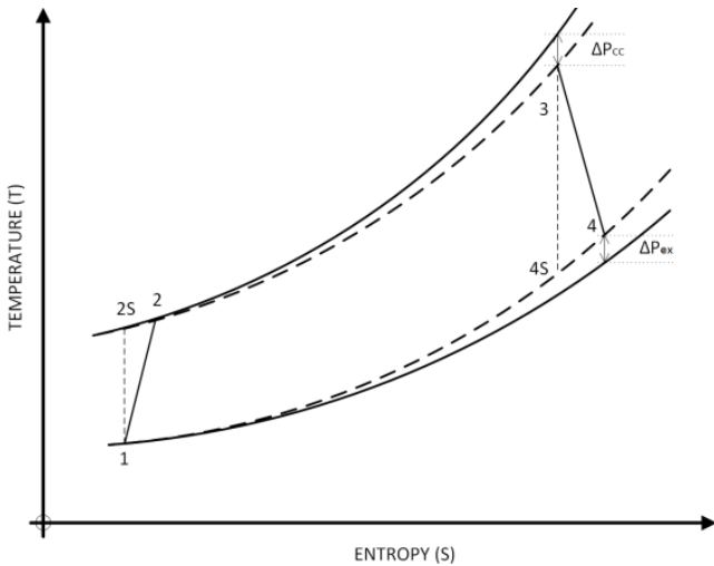
Fig. 2 Temperature-entropy diagram
