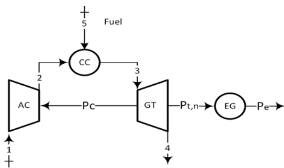
Fig. 1 Schematic diagram of the selected GT unit
