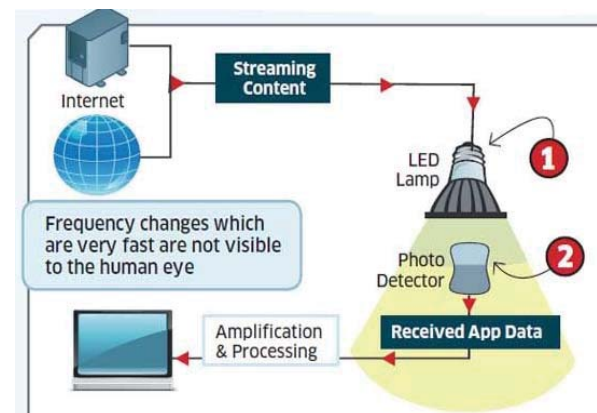
Fig. 4 Overall Design of Li-Fi [4]
