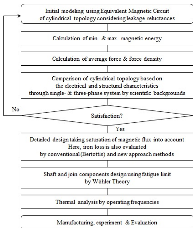
Fig. 1 Analysis Flow
