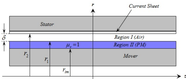
Fig. 8 Analytical Field Model
