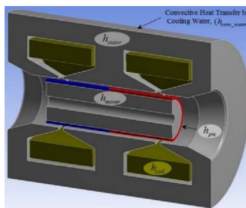
Fig. 12 Cylindrical Topology with Heat Generation
