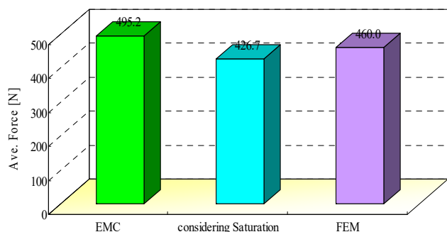
Fig. 9 Comparison of Average Force by Calculation Methods
