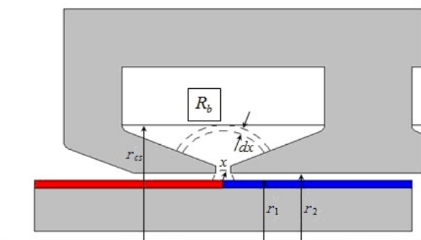
Fig. 4 Permeance at Maximum Position
