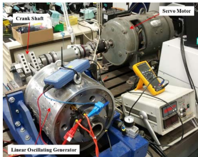
Fig. 14 Test Environment for Measurement
