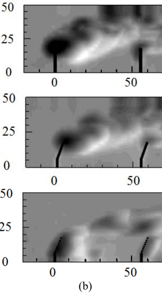
Fig. 5 (a) Flow fields and (b) bed topography due to spurs of different configuration
