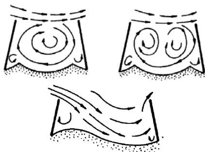
Fig. 3 Flow pattern in a spur-field as in [24]
