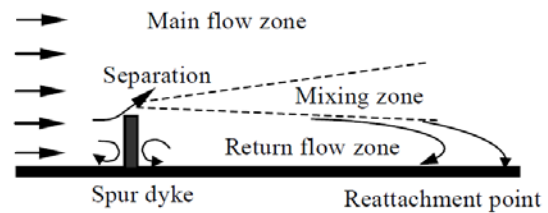
Fig. 2 Flow zones due to a spur [20]
