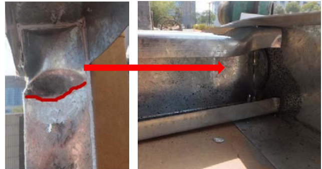
(a) Distortional buckling of W-1 CFS
