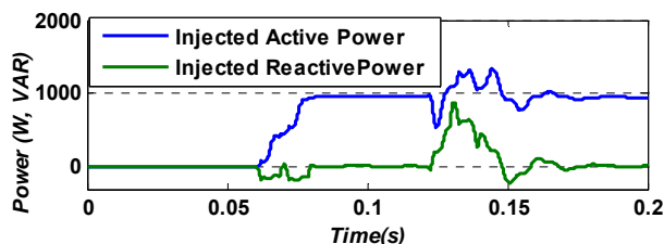
Fig. 11 Injected active & reactive power profiles with and without the active filter
