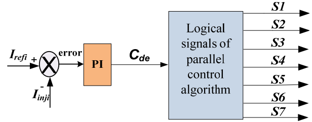
Fig. 4 Control block by the PI controller
