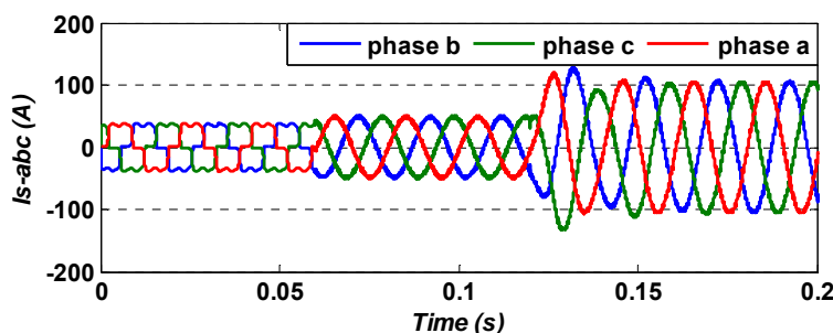
Fig. 9 Three-phase supply currents waveforms after filtering
