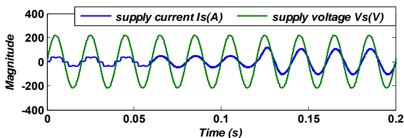
Fig. 8 Power Factor
