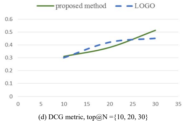
Fig. 4 The results of evaluation metrics for comparing the performance of proposed method
