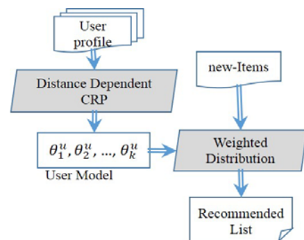
Fig. 1 The proposed model for recommender system
