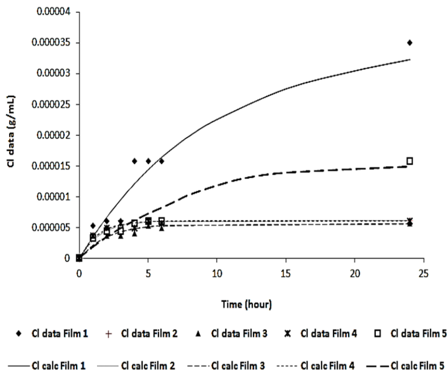
Fig. 5 Comparison between Cl data and Cl Calculate with Loading Time 12 hours
