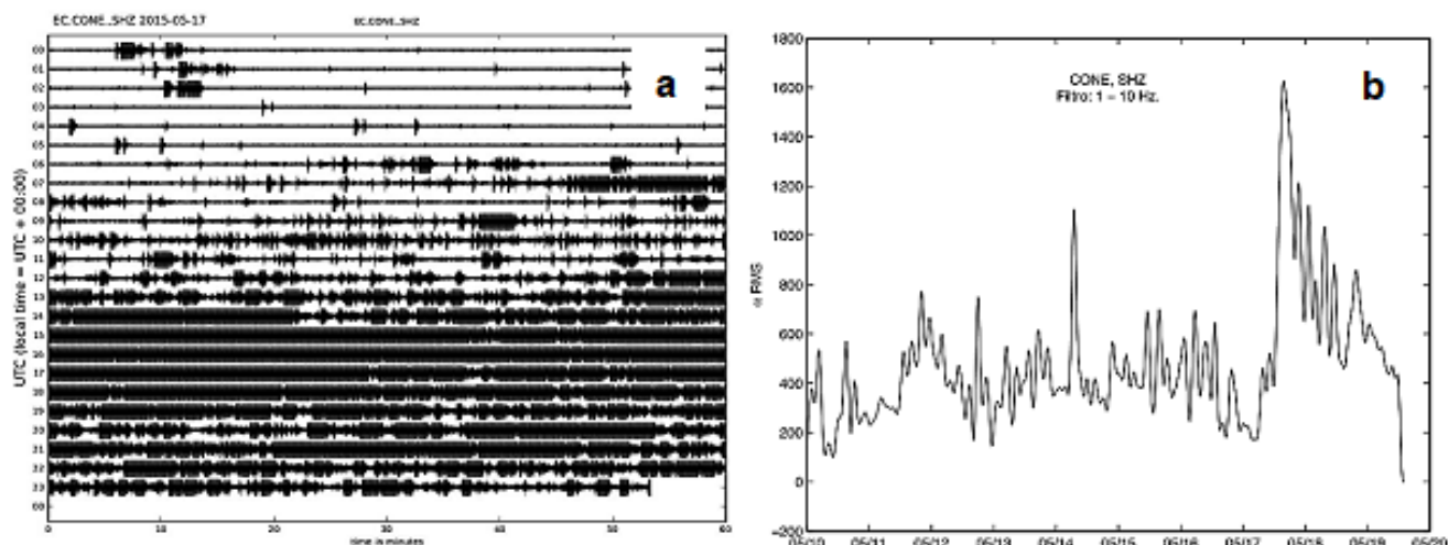
Fig. 4 (a) Seismogram of the CONE station, which is located at the NE flank, shows an important and sustained increase in the tremor's amplitude since 13h50 UTC on 17 May. (b) Evolution of the seismic amplitudes recorded from 10/05/2015 – 19/05/2015, noticing an important increase on 17 May amplitudes and a posterior decrease. Taken and edited from [10]
