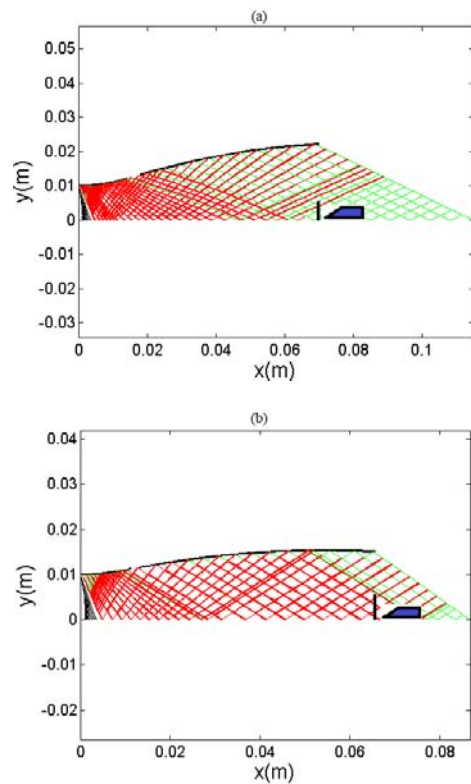
Fig. 2 Rotation of Mach 2 nozzle wall keeping the throat constant, and the wall is rotated by an angle (a) \Omega = 3.5^\circ and \Omega = -2.5^\circ .
