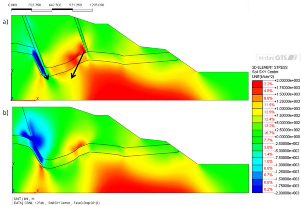
Fig. 9 Shear stress distribution (a) considering and (b) not considering the presence of fracture zones along faults
