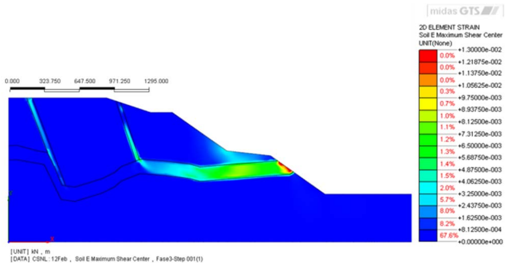
Fig. 10 Failure surface associated with DSGSD deformation
