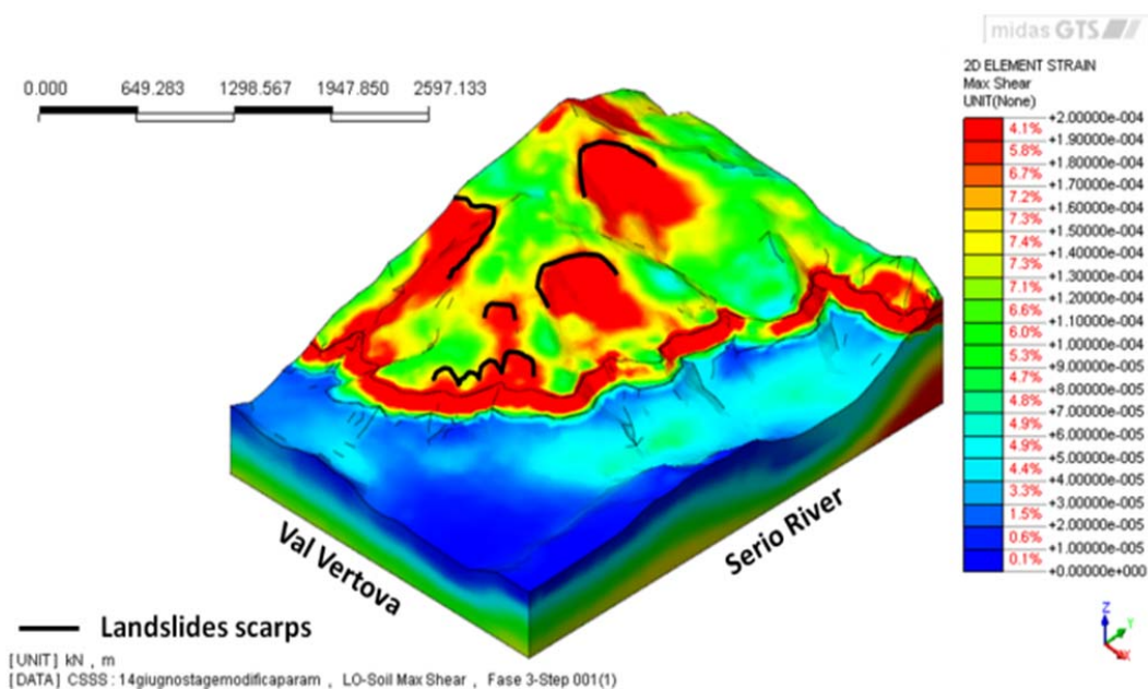
Fig. 16 3D shear strain distribution
