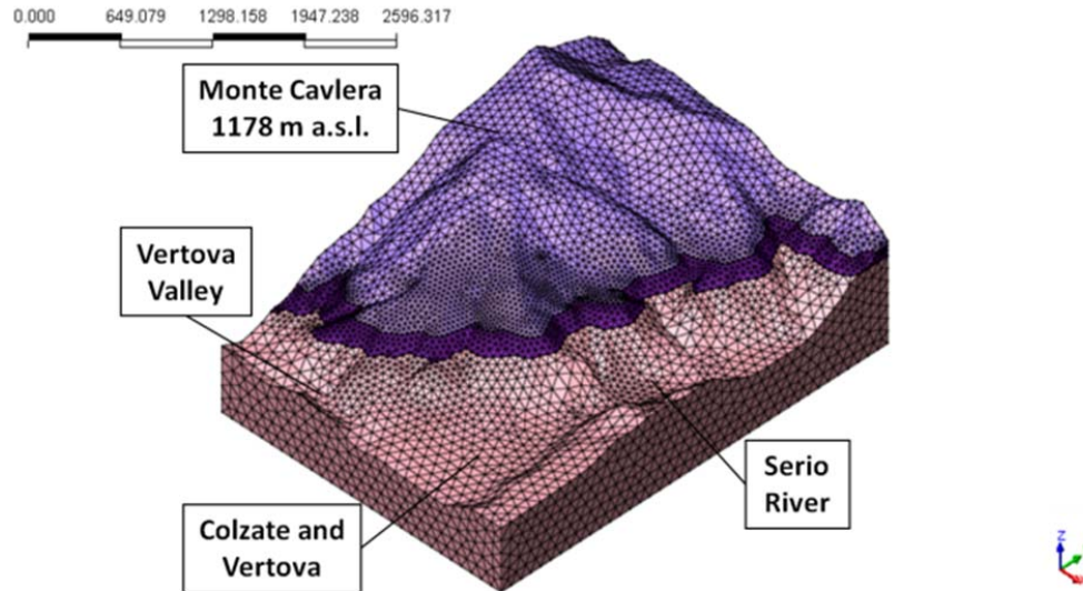
Fig. 13 3D domain and its mesh
