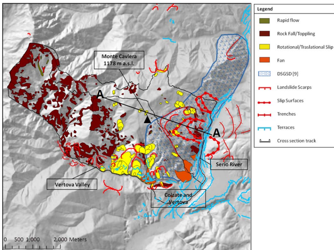
Fig. 2 Geomorphological map
