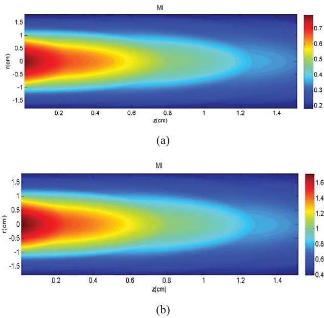
Fig. 2 Ultrasound MI contour of 40 kHz in the r-z, intensity of (a) 0.28 W/cm 2 , (b) 1.34 W/cm 2 : The vertical axis (r) and the horizontal axis (z) show the radial and axial lengths in cm; Color map from blue to red indicates increase in MI
