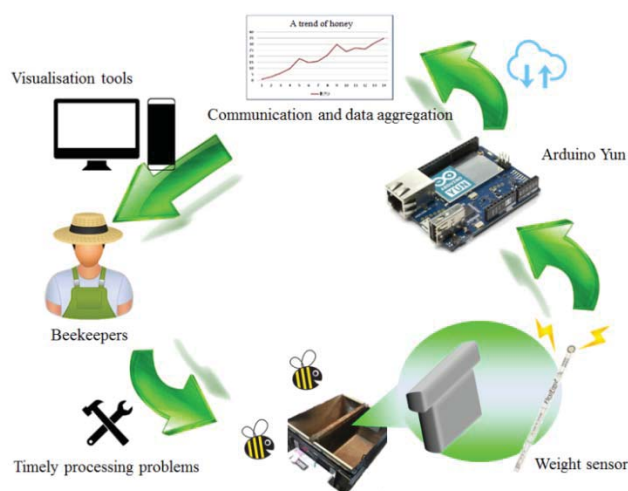
Fig. 1 Architecture of the weighing system
