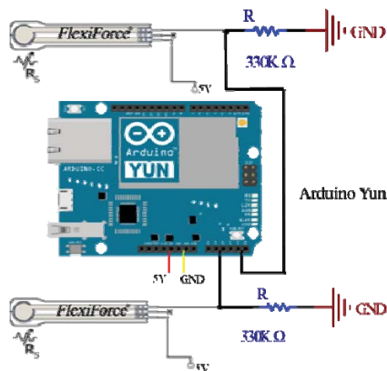
Fig. 5 The main circuit of the system
