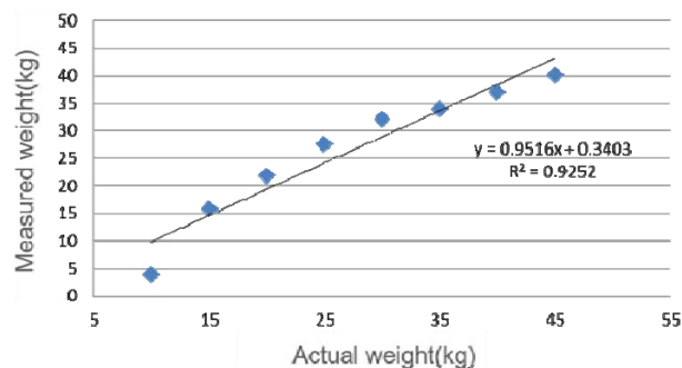
Fig. 10 Average measured weight compared with the actual weight in the regular case
