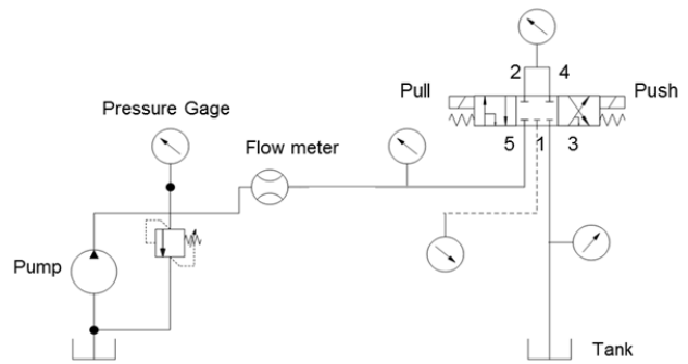
Fig. 12 System schematic of the test setup
