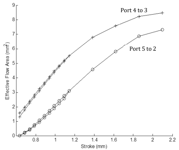
Fig. 9 Effective flow area for both of the flow paths obtained by CFD analysis
