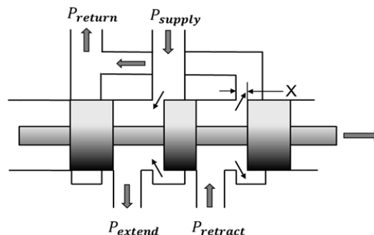
Fig. 1 Detail of spool shown in Fig. 2 [7]
