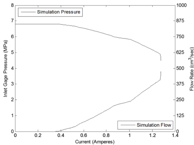
Fig. 14 Simulation results for modified spool geometry
