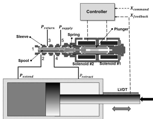
Fig. 2 Solenoid-driven spool valve geometry and schematic
