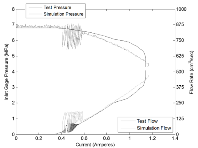
Fig. 13 Simulation and test results showing flow oscillations
