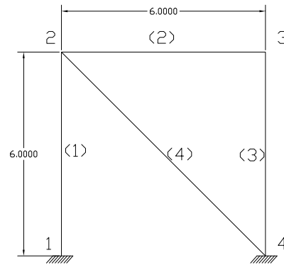
Fig. 3 The fame with 4 members
