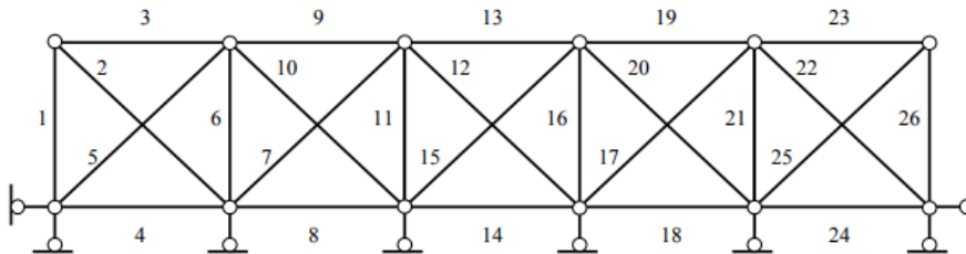
Fig. 2 The truss with 26 members
