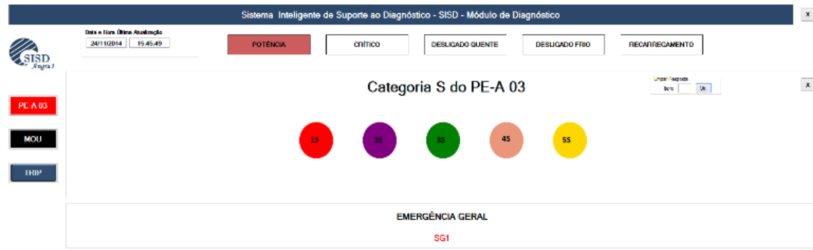
Fig. 9 Class classification
