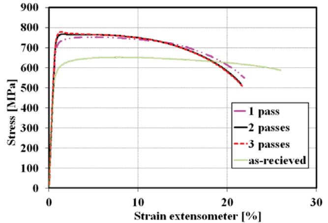
Fig. 11 Engineering stress-strain curves in different structural states for Ti Grade 4
