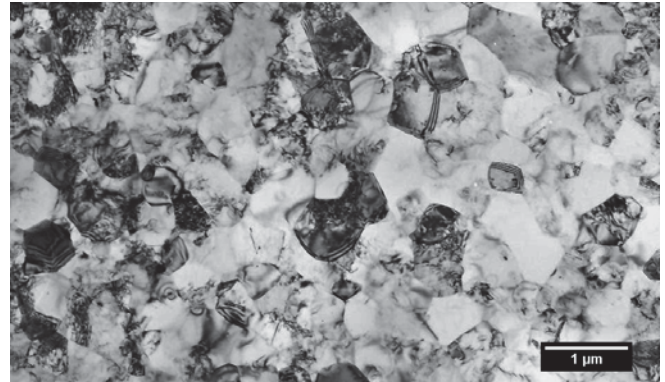
Fig. 7 The structure of Ti Grade 4 upon three passes through CONFORM SPD; the mean grain size is 435 \pm 195 nm
