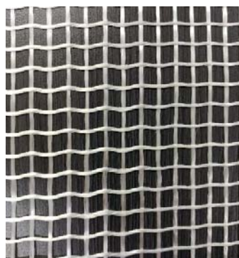
Fig. 1 AR-glass textile of 640tex
