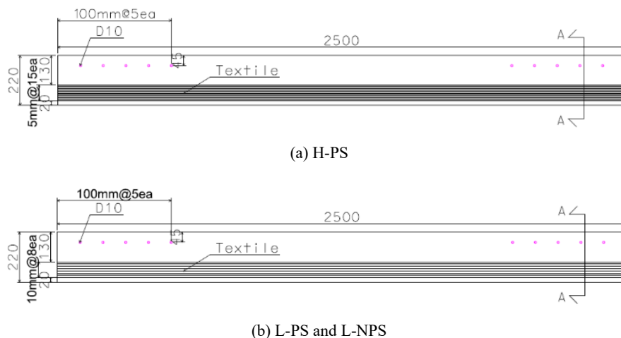
Fig. 2 Detail specification of tested TRC specimen
