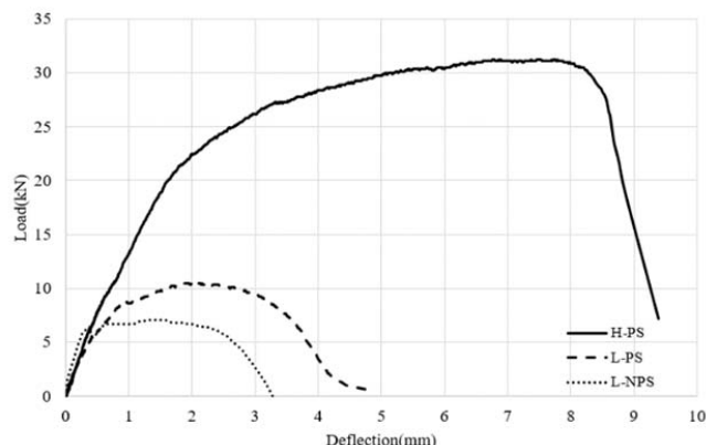
Fig. 6 Load and displacement curve of TRC specimen
