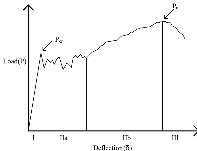
Fig. 7 General behavior of thin TRC member
