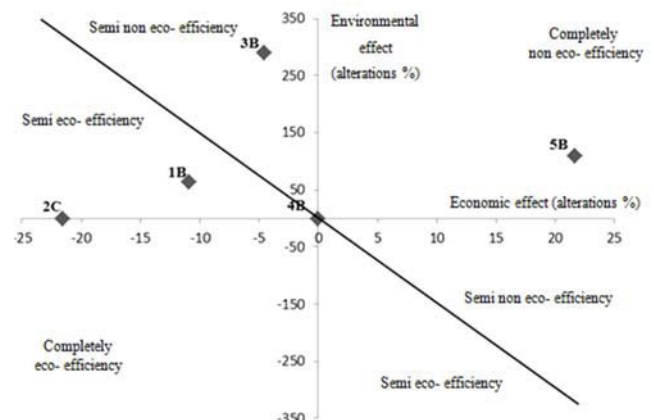
Fig. 9 Eco-efficiency diagram of environmental top scenarios
