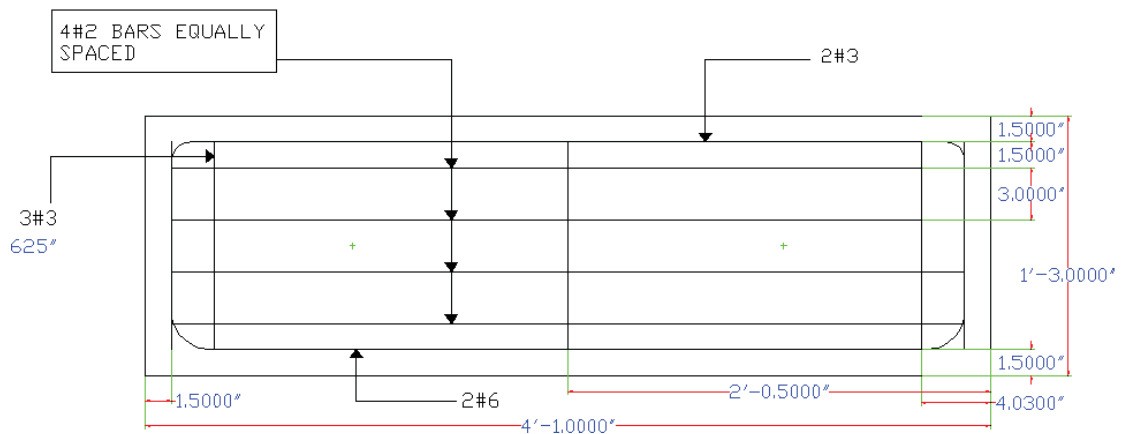
Fig. 6 Reinforcement details of 381mm (15in) deep beam
