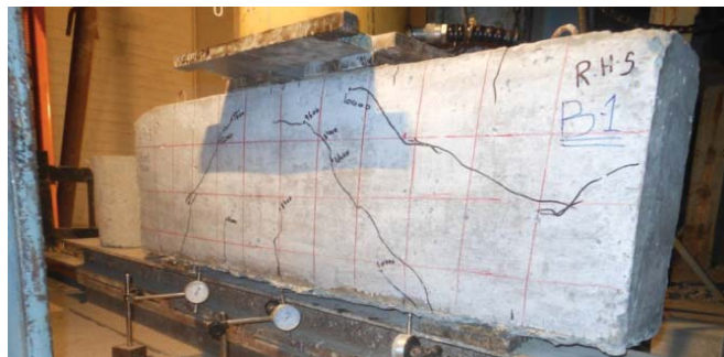
Fig. 8 381mm (15in) deep beam crack pattern
