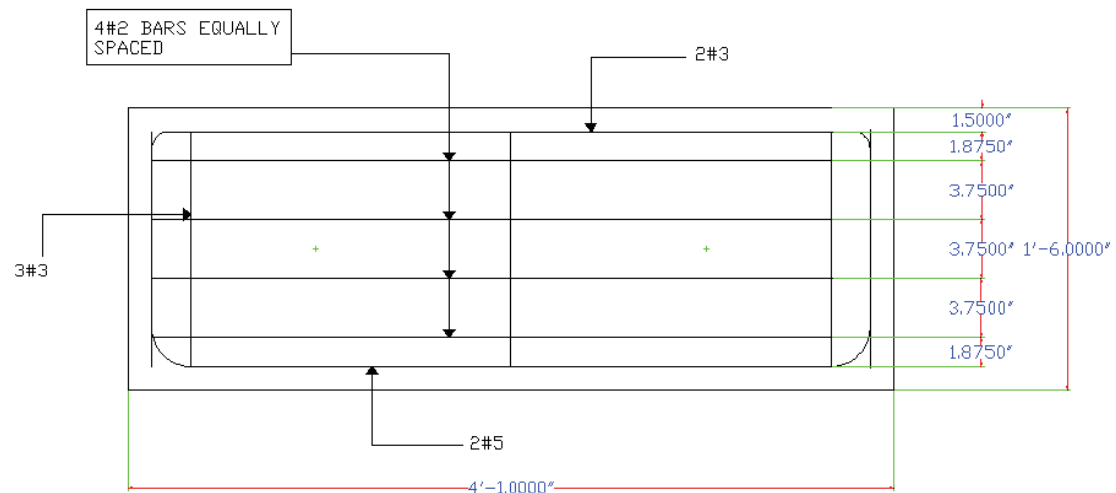
Fig. 7 Reinforcement details of 457mm (18in) deep beam
