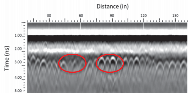
Fig. 3 GPR B-Scan
