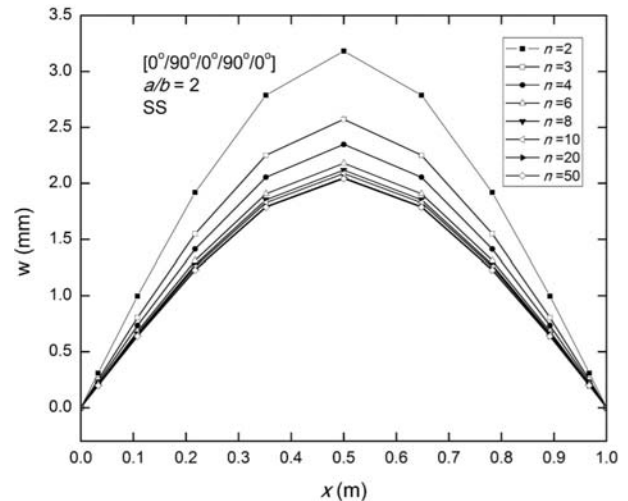
Fig. 7 Transverse displacement values of super-elliptic beam with different ovality values for SS boundary condition ( a/b=2 , [0^\circ/90^\circ/0^\circ/90^\circ/0^\circ] )
