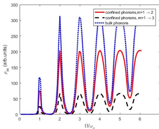
Fig. 2 Dependence of MR \rho_{xx} on \Omega/\omega_c
