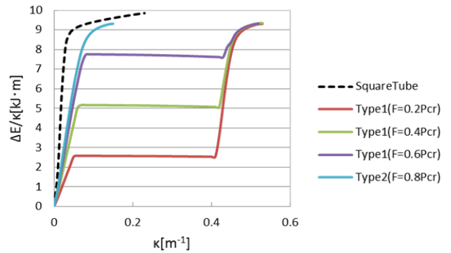
Fig. 18 Energy comparisons at various F rate
