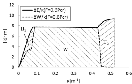
Fig. 20 Comparison energy between F=0,2P_{cr} and F=0,6P_{cr}
