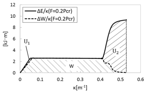
Fig. 19 Different energy characteristics in type 1 and 2
