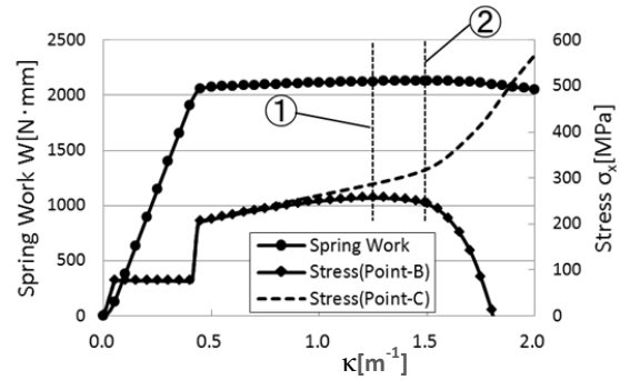
Fig. 11 Flat collapse mechanisms
