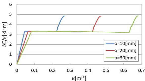
Fig. 21 Energy characteristic due to change x amount
