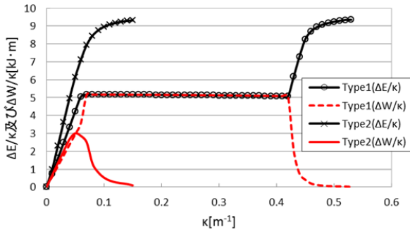
Fig. 19 Different energy characteristics in type 1 and 2
