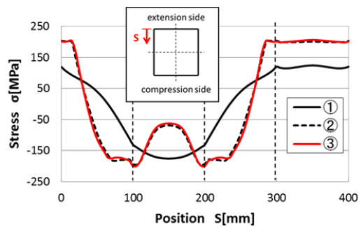
Fig. 8 Cross-sectional stress of side collapse
