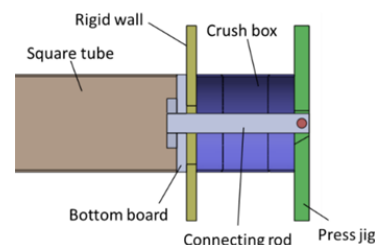
Fig. 1 Square tube model
