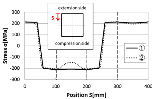
Fig. 10 Cross-sectional stress of bottom collapse
