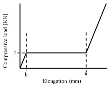
Fig. 3 Absorption part characteristic
