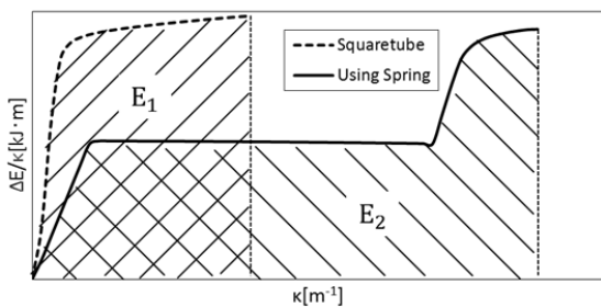
Fig. 15 Influence of spring at square tube bending
