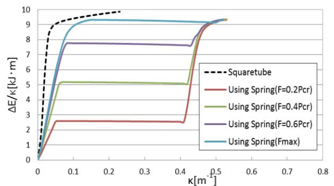
Fig. 22 Increase total energy using F_{max}
