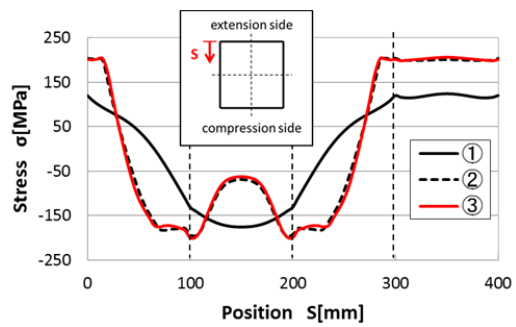
Fig. 8 Cross-sectional stress of side collapse
