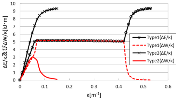
Fig. 19 Different energy characteristics in type 1 and 2
