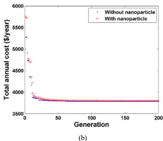
Fig. 2 Progress of objective function versus generation for two cases of without/with additive nanoparticle (a) m_w=2 kg/s, (b) m_w=6 kg/s
