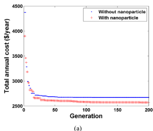
Fig. 1 Progress of objective function versus generation for two cases of without/with additive nanoparticle ( m_w=4 kg/s)
