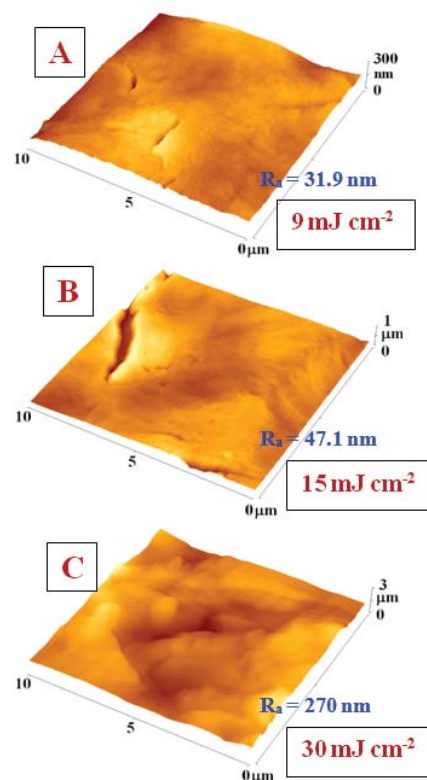
Fig. 4 3D AFM scans of PHB laser treated by 6000 pulses and different laser fluence – 9 (A), 15 (B) and 30 (C) \text{mJ cm}^{-2} . Ra represents arithmetic mean roughness
