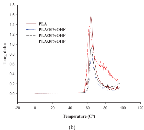
Fig. 5 Variation of storage modulus ( E' ) and \text{Tan } \delta of PLA and composites as function of temperature
