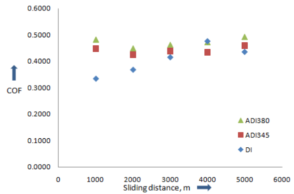
Fig. 3 COF as a function of sliding distance
