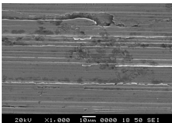
Fig. 11 SEM image of worn surface of ADI380
