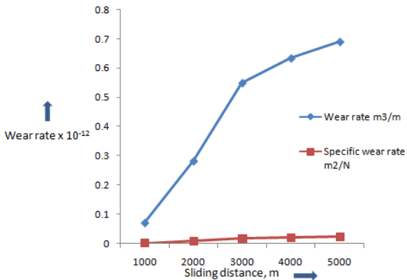
Fig. 6 Wear rate and specific wear rate of ADI345
