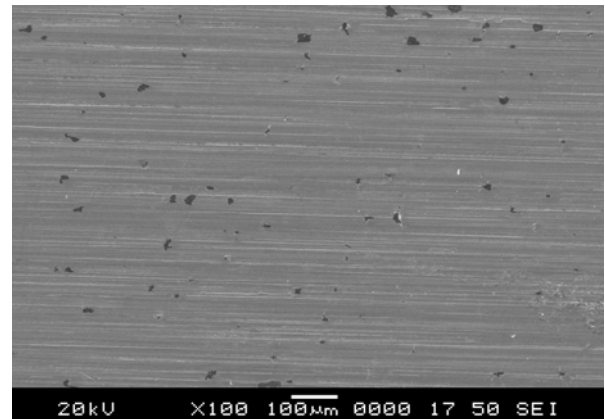
Fig. 8 SEM image of ADI345
