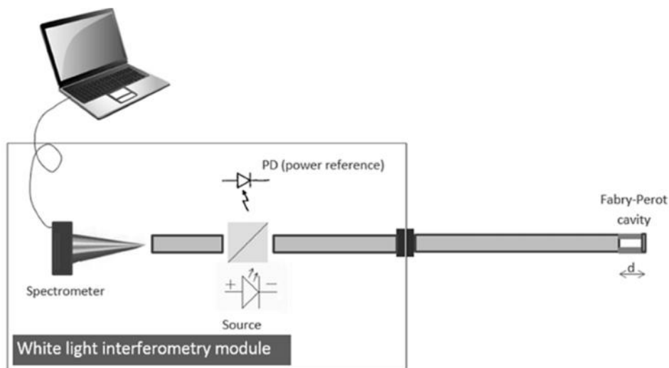
Fig. 5 A concept for an optical pressure sensor
