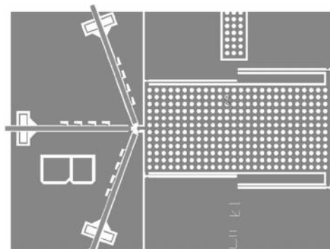
Fig. 1 MEMS optical accelerometer layout
