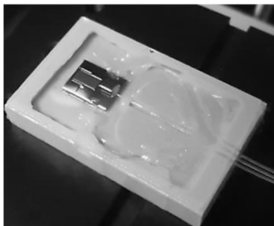
Fig. 8 Assembled accelerometer chip with the fibres
