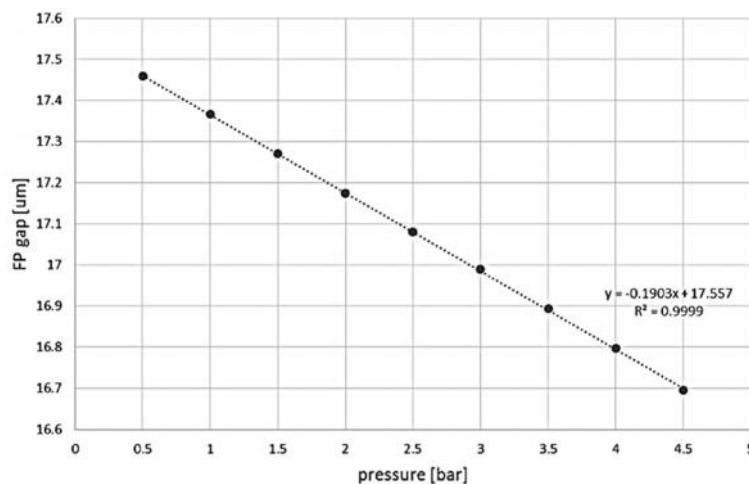
Fig. 12 Fabry-Perot gap vs chamber pressure
