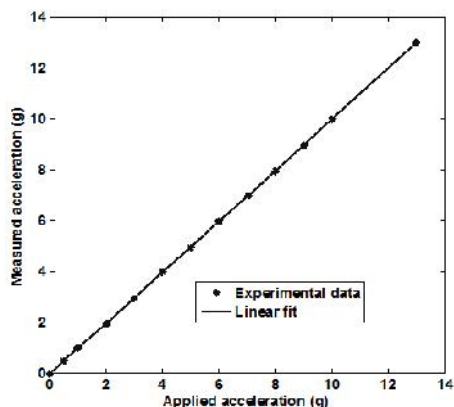
Fig. 10 Performance of one specific optical MEMS accelerometer
