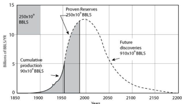
Fig. 1 Hubert's Curve
