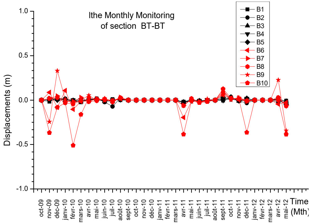
Fig. 4 Displacement of topographic point according to cut BT-BT
