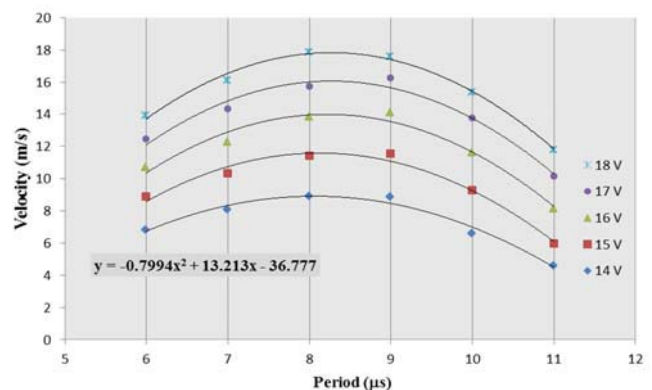
Fig. 1 Droplet velocity as T_{keep} function
