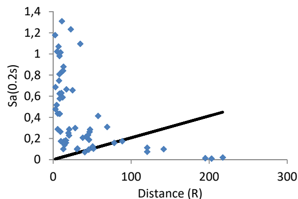
Fig. 5 Sufficiency of Sa(0.2s) for Distance R
