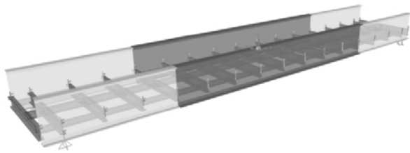
Fig. 1 3D extrude view of bridge model
