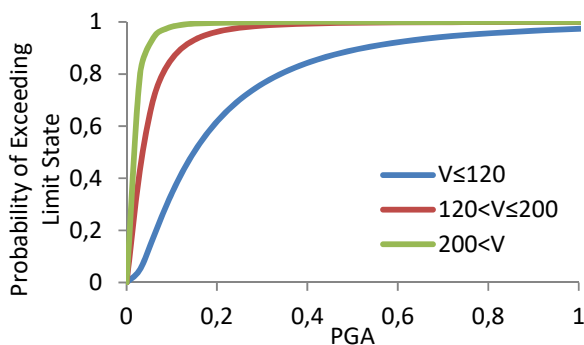
Fig. 7 Probability of Exceeding Lateral Displacement Limit State
