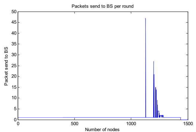
Fig. 7 Throughput of the network for Eo = 0.5
