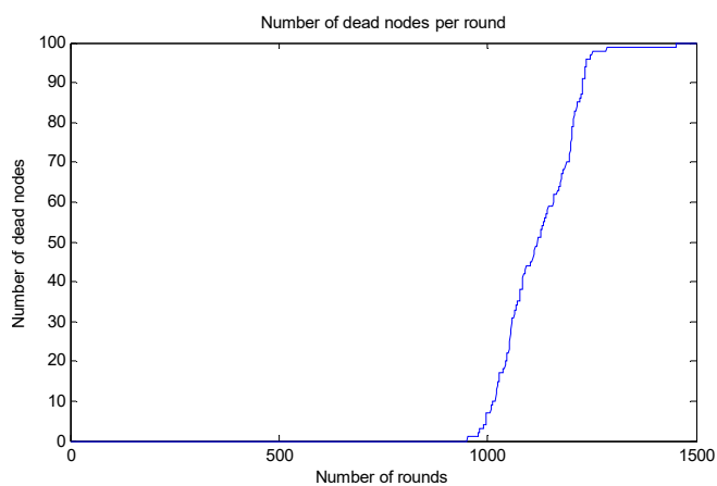
Fig. 5 Number of dead node for Eo = 0.5
