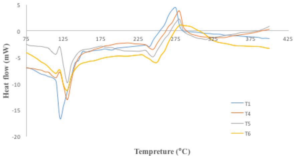
Fig. 2 DSC Thermograms of different ratio of CS:EO. (T2 and T3 not determined)
