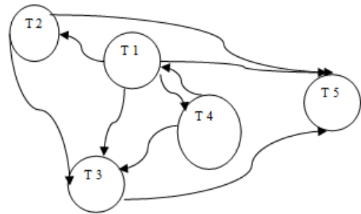
Fig. 2 Leagility Digraph
