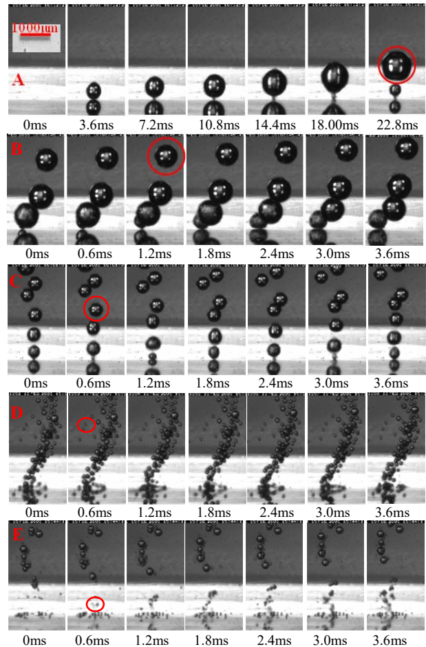
Fig. 6 Micro-bubble formation processes images at different driving resonance frequencies (A) 0 kHz, (B) 12.5 kHz, (C) 28.13 kHz, (D) 76.25 kHz, (E) 130.6 kHz, with inlet gas pressure of 25.5 kPa
