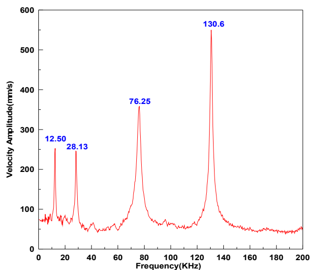
Fig. 3 Frequency response of the vibrating piezoelectric transducer
