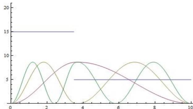
Fig. 2 Free particle confined in an infinite square well potential. The probability density |\psi_n(x)|^2 , n = 1, 2, 3 in (31) and the mass distribution m(x) given in (28). m_1 = 15 , m_2 = 5 , x_0 = 3.5 and \hbar = m_0 = 1
