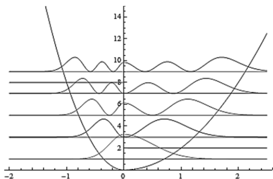
Fig. 3 Potential (32), the probability density |\psi_n(x)|^2 given in (33), the energy spectra E_n = \beta(2n + 1) , n = 0, 1, 2, 3, 4 and the mass distribution m(x) given in (28). m_1 = 8, m_2 = 2, x_0 = 0, \beta = 1 and \hbar = m_0 = 1
