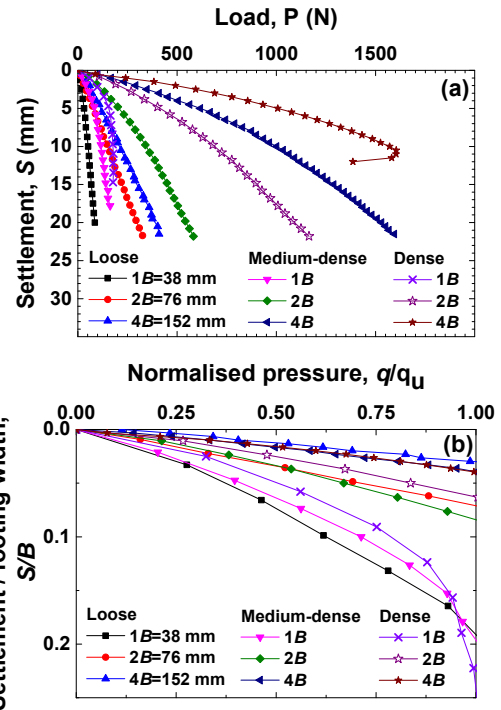
Fig. 3 (a) Load-settlement (b) Normalised pressure-strain curves for different width of footings on loose, medium-dense and dense sand
