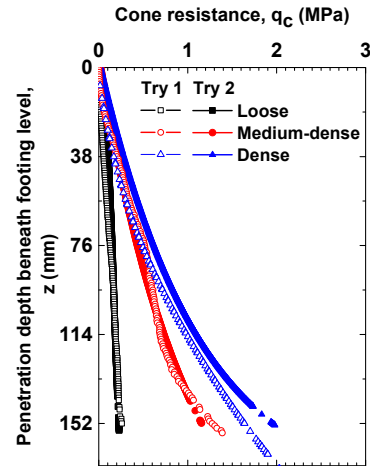
Fig. 1 CPT data for the sand packing
