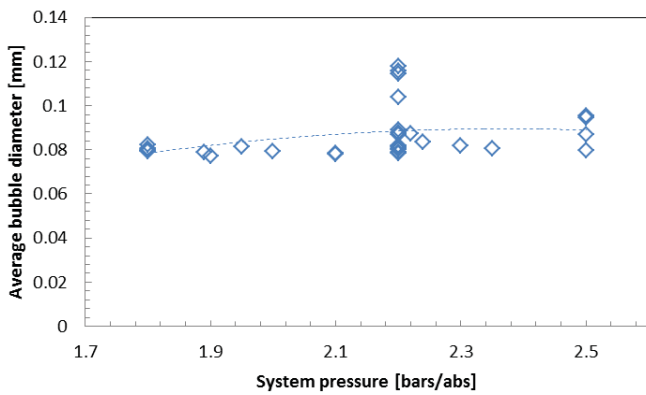
Fig. 9 Experimental bubble diameters with the system pressure
