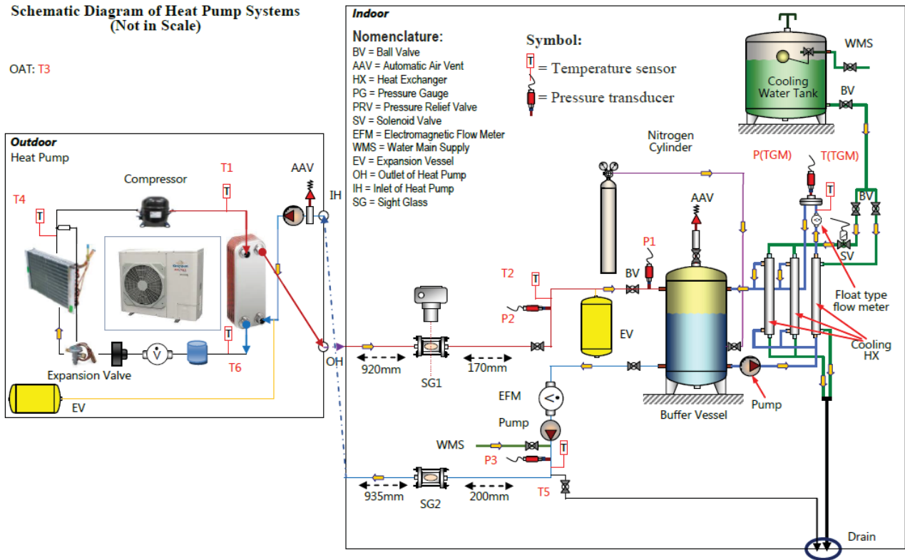
Fig. 2 Schematic diagram of heat pump system
