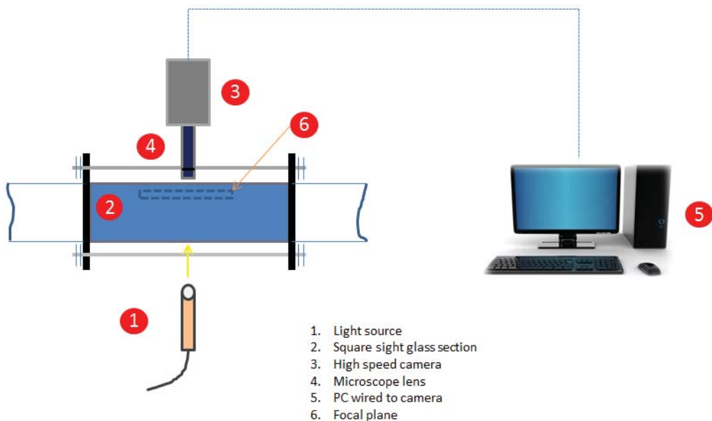
Fig. 3 Horizontal sight-glass for bubble capturing
