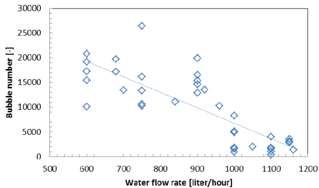
Fig. 12 Bubble number with water flow rate during 3 minutes
