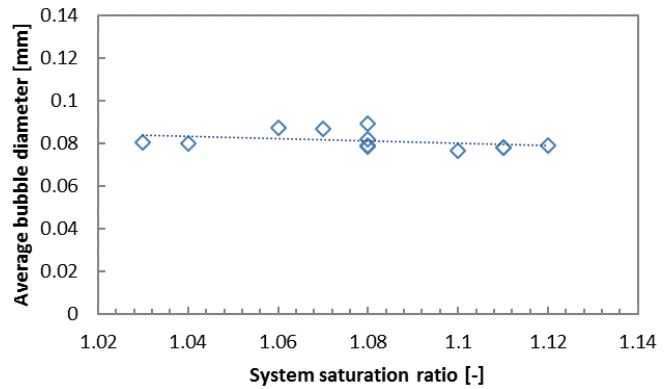
Fig. 11 Experimental average bubble diameters with SR
