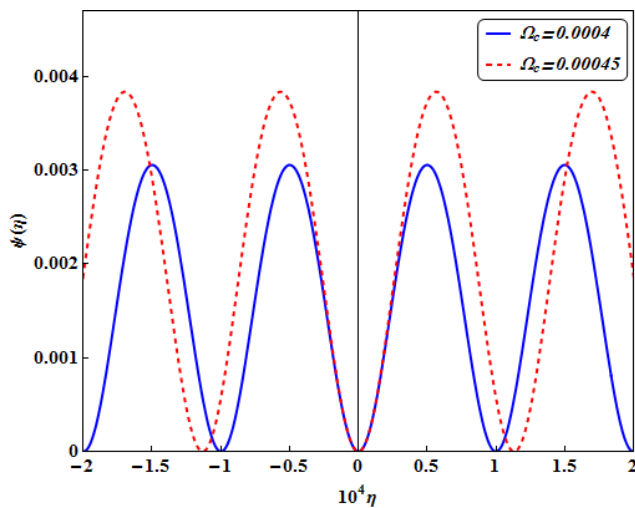
Fig. 8 Variation of periodic travelling wave \Psi versus \eta for \chi = 2 , \delta = 0.2 , l_x = 0.2 , \gamma_{xe,p} = 0.4 , \lambda_{xe,p} = 0.1 and U = 0.4
