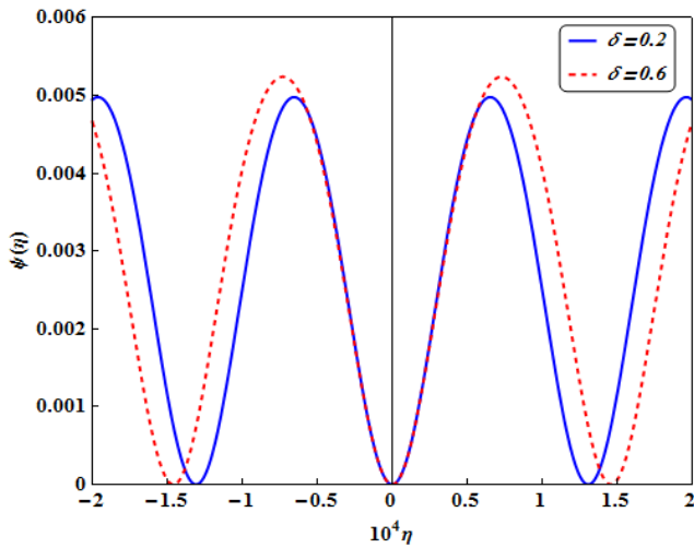
Fig. 7 Variation of periodic travelling wave \Psi versus \eta for \chi = 2 , l_x = 0.4 , \gamma_{xe,p} = 0.4 , \lambda_{xe,p} = 0.1 , U = 0.4 and \Omega_c = 0.004
