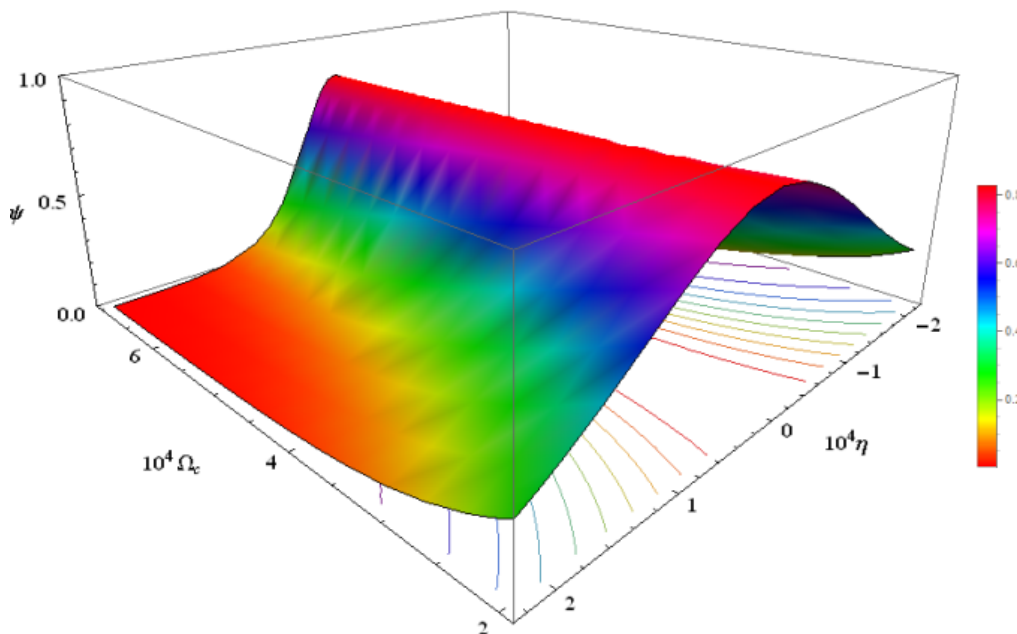
Fig. 5 The variations of solitary wave versus \Omega_c with \delta = 0.2 , \gamma_{xce,p} = 0.4 , \lambda_{xce,p} = 0.1 , l_x = 0.4 and U = 2.17 .
